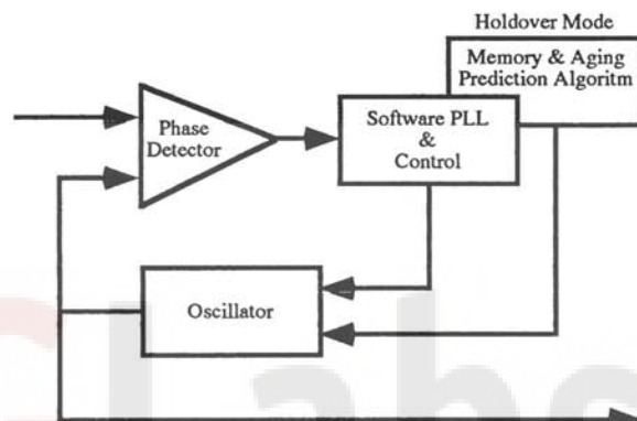
Figure 1. HP SmartClock Concept
