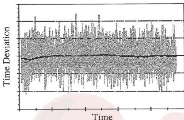
Figure 3. Enhanced GPS filtering reduces SA jitter from about 300 ns to 50 ns RMS
