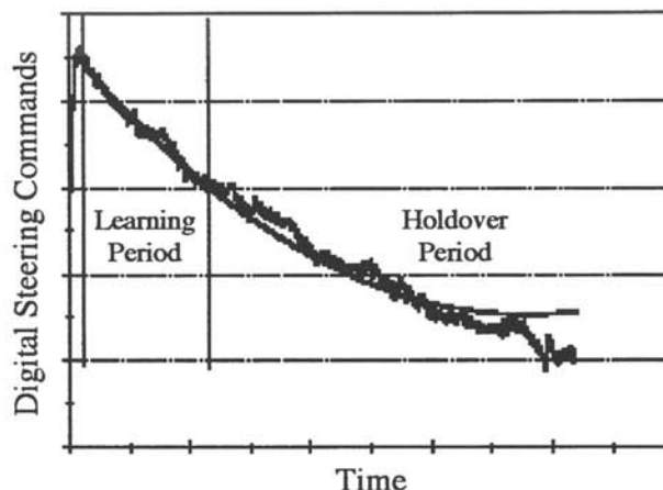
Figure 2. Typical HP SmartClock Holdover Aging Performance
